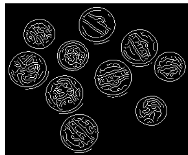
Canny Filter
