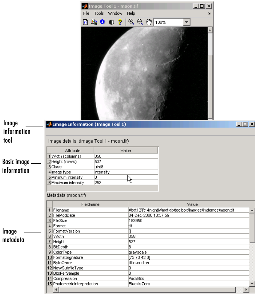
Image Tool with Image Information Tool
