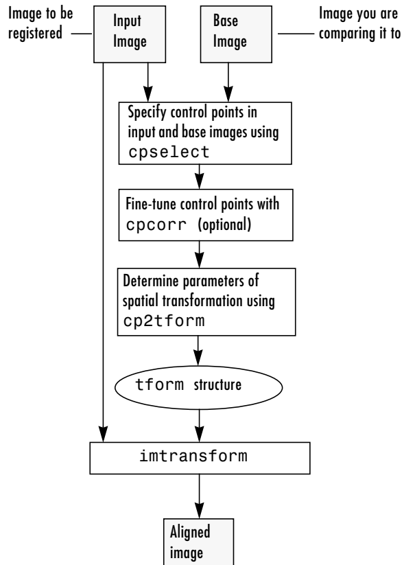
Overview of Image Registration Process
