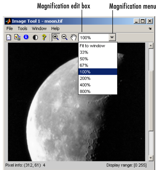
Image Tool Magnification Edit Box and Menu
