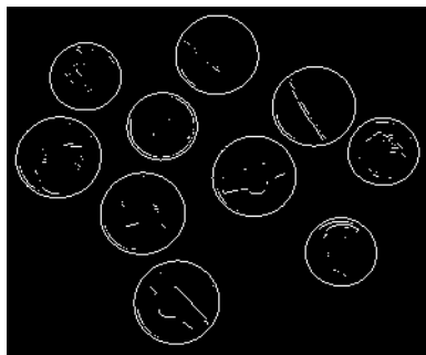
Sobel Filter
